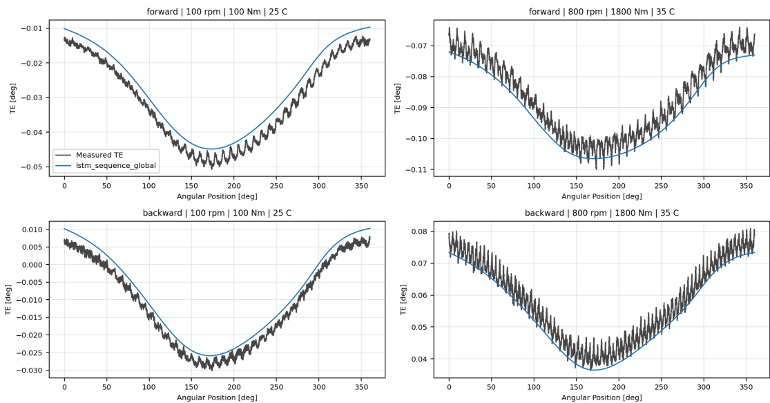
lstm_sequence_global Track 2 collage
