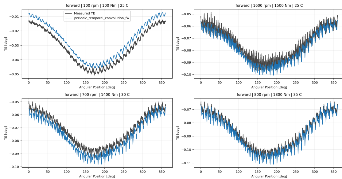
periodic_temporal_convolution_fw Track 2 collage
